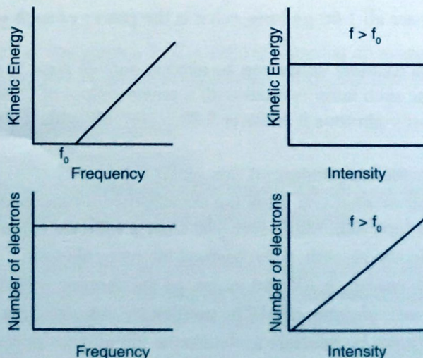
Figure 12.3: Characteristics of the photoelectric effect
